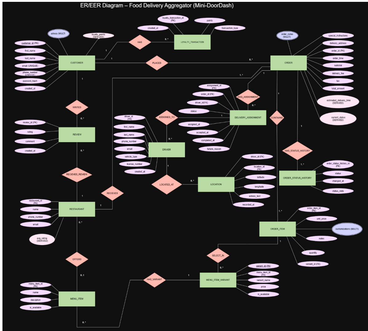
Figure 1. Comprehensive ER/EER Diagram – Food Delivery Aggregator (Mini-DoorDash)
